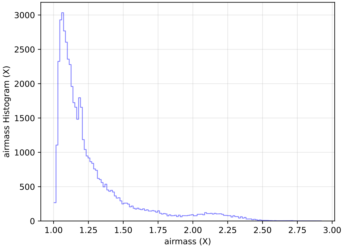
reweight_plane_v3.3_10yrs Yr 1 r band: airmass Histogram
