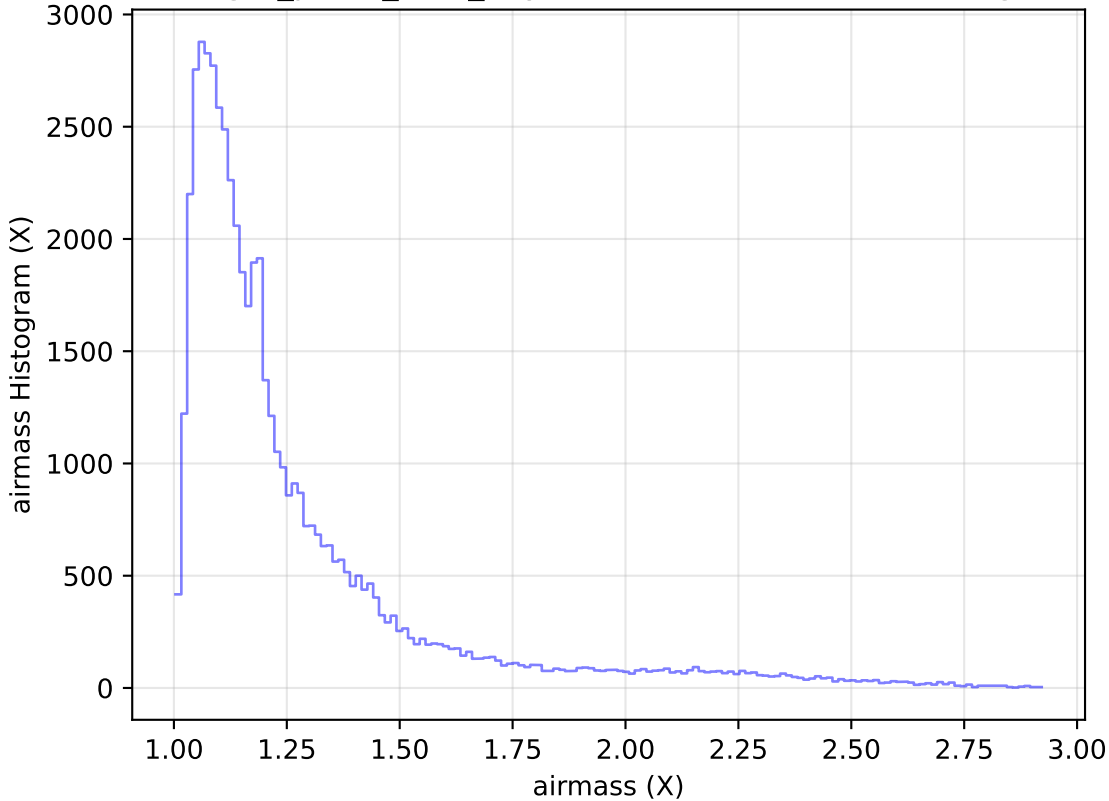
reweight_plane_v3.3_10yrs Yr 1 i band: airmass Histogram
