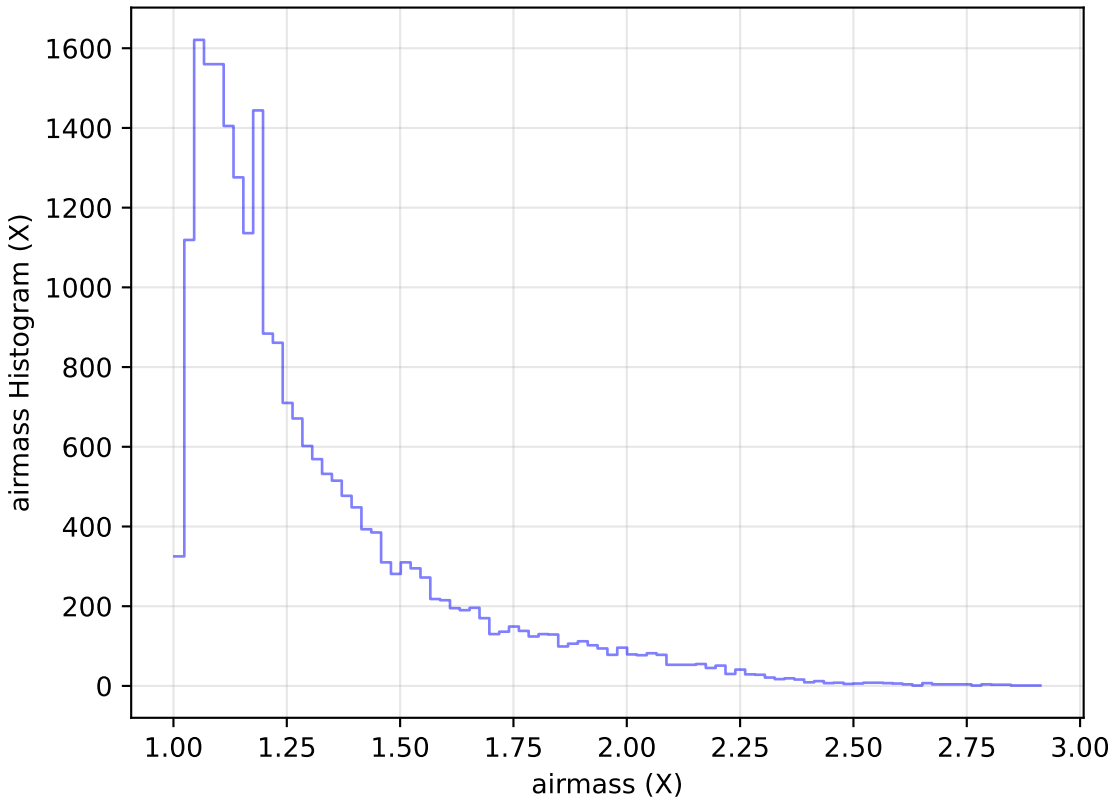
reweight_plane_v3.3_10yrs Yr 1 g band: airmass Histogram
