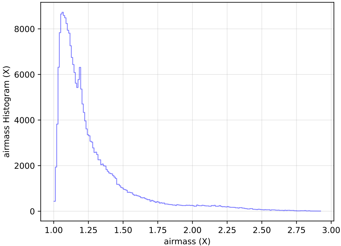
reweight_plane_v3.3_10yrs Yr 1 all bands: airmass Histogram
