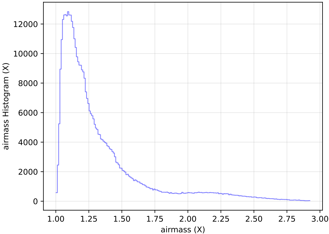
reweight_plane_v3.3_10yrs WFD z band: airmass Histogram
