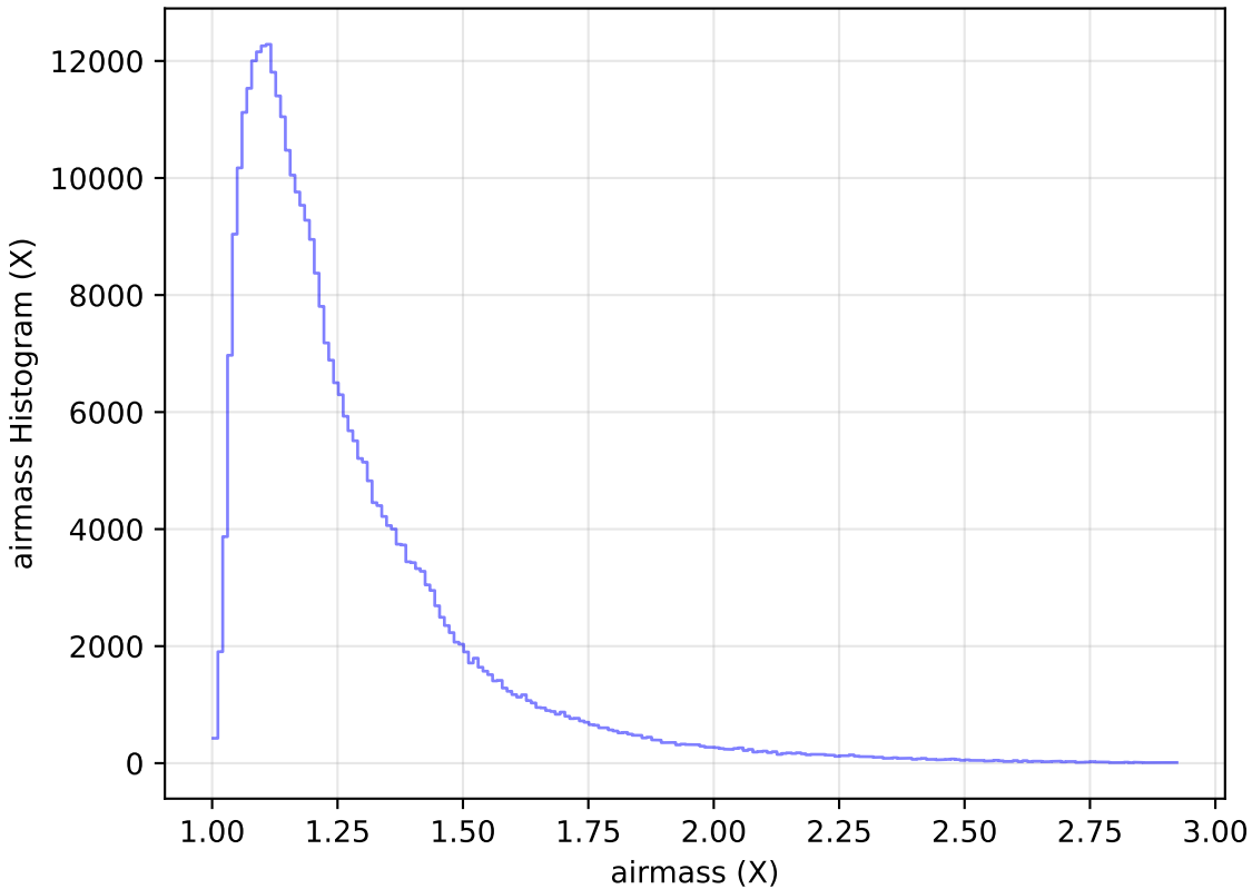
reweight_plane_v3.3_10yrs WFD y band: airmass Histogram
