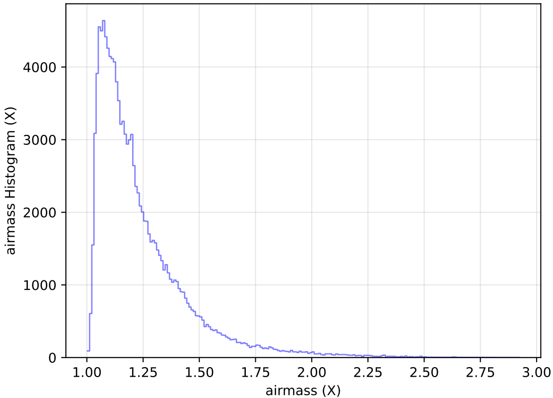
reweight_plane_v3.3_10yrs WFD u band: airmass Histogram
