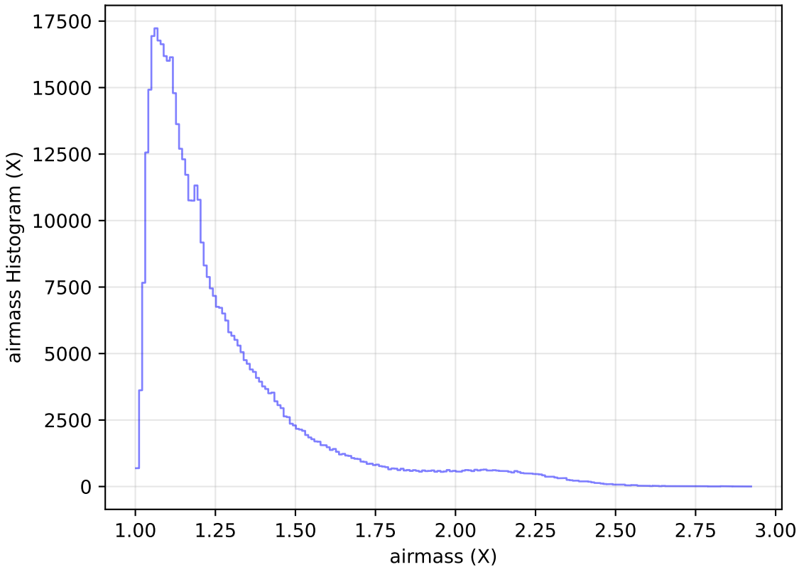
reweight_plane_v3.3_10yrs WFD r band: airmass Histogram
