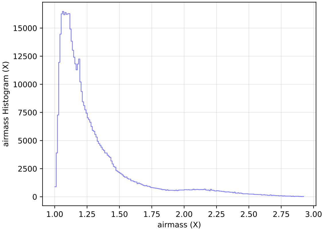
reweight_plane_v3.3_10yrs WFD i band: airmass Histogram
