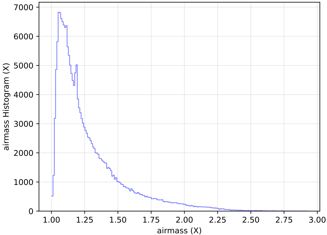
reweight_plane_v3.3_10yrs WFD g band: airmass Histogram
