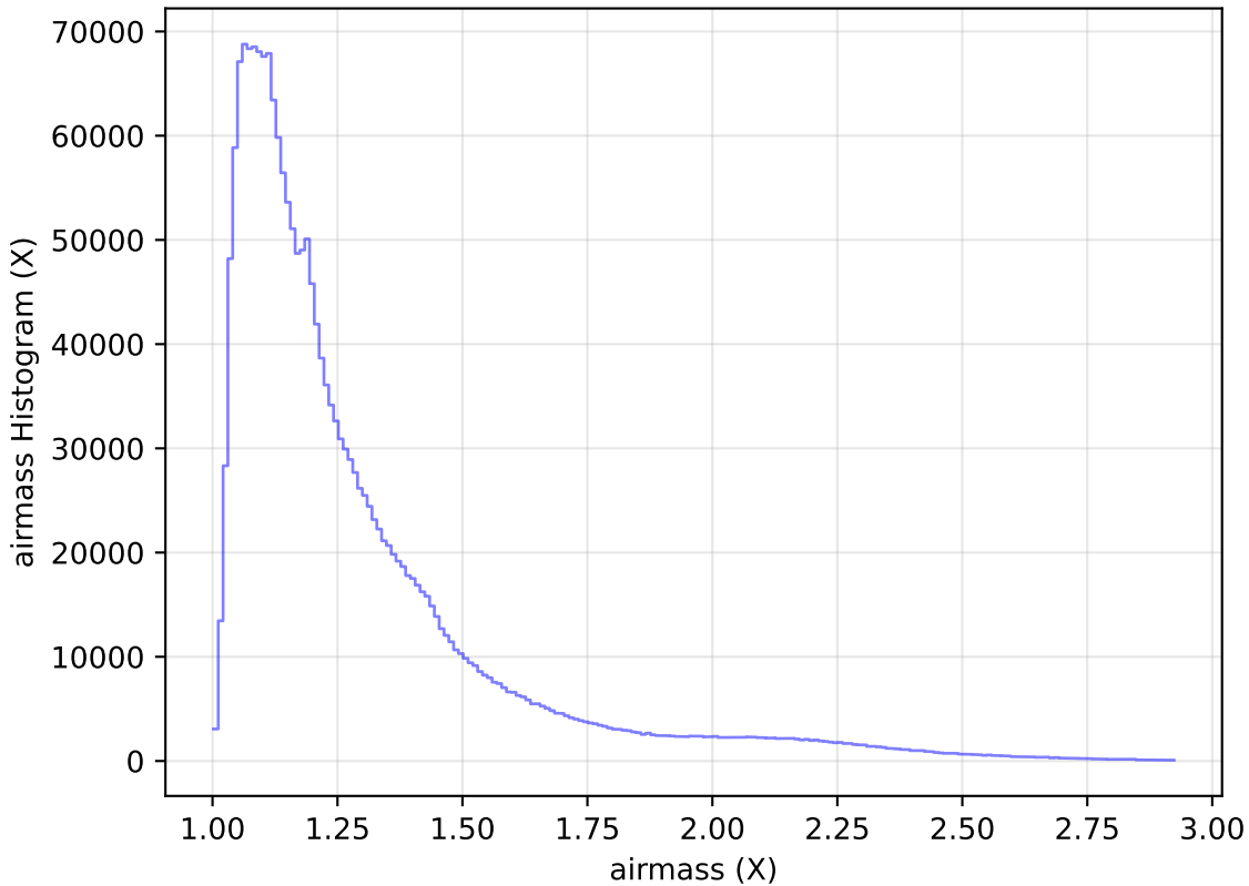
reweight_plane_v3.3_10yrs WFD all bands: airmass Histogram
