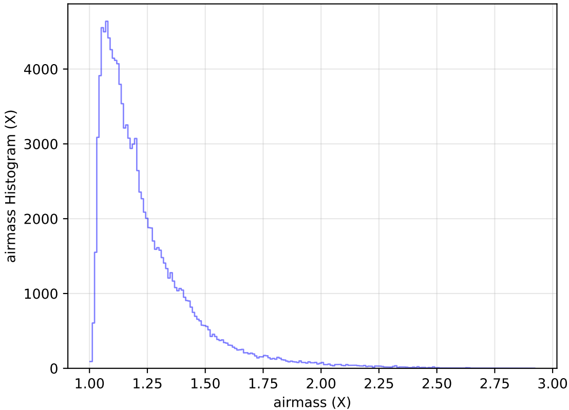
reweight_plane_v3.3_10yrs All sky u band: airmass Histogram
