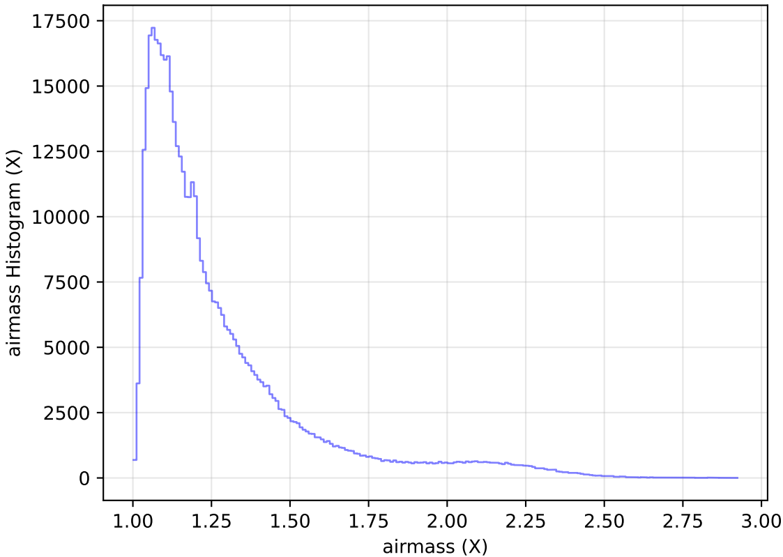
reweight_plane_v3.3_10yrs All sky r band: airmass Histogram
