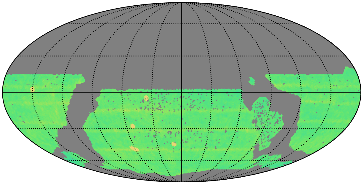
reweight_plane_v3.3_10yrs WFD all bands: N Unique Nights
