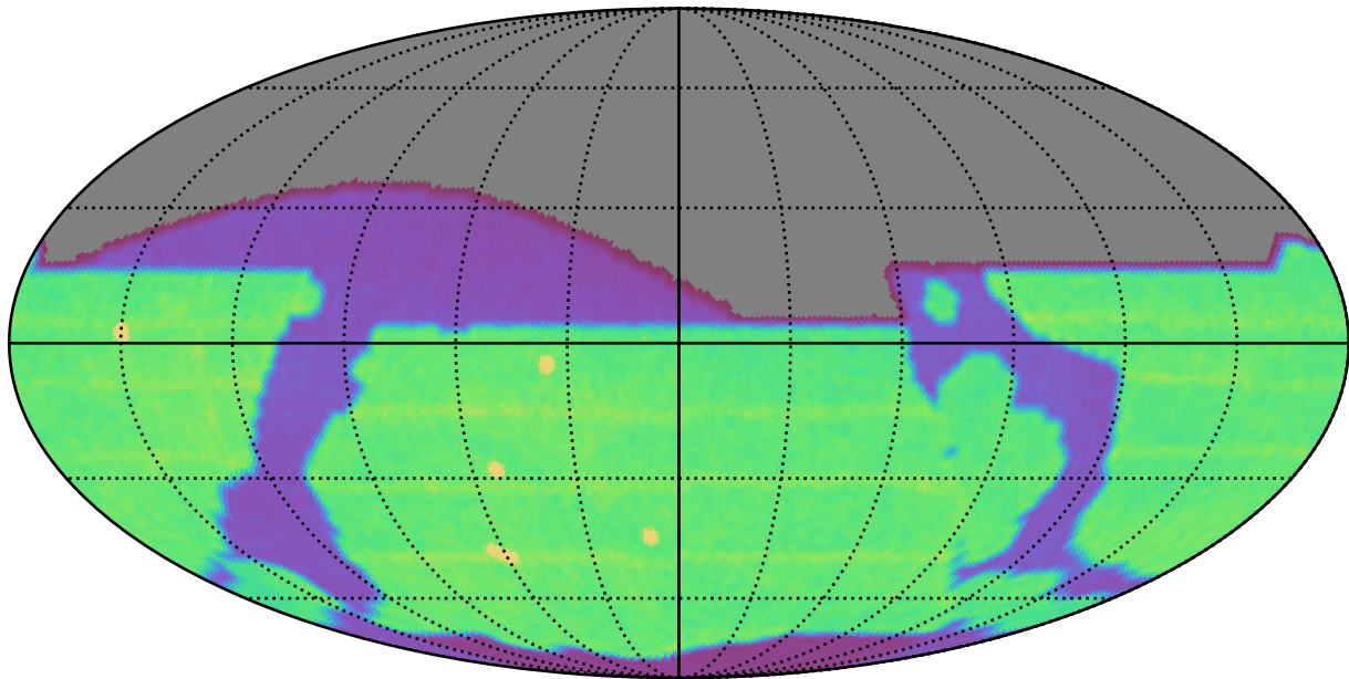
reweight_plane_v3.3_10yrs All sky all bands: N Unique Nights
