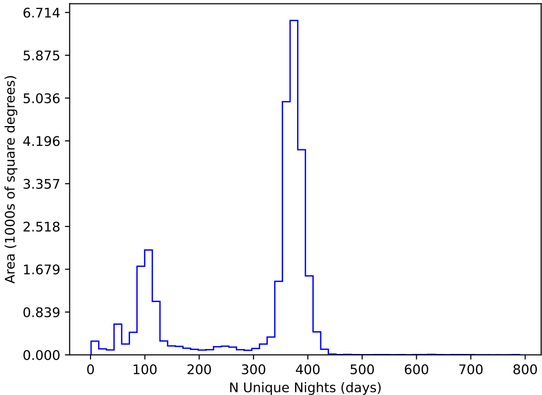
reweight_plane_v3.3_10yrs All sky all bands: N Unique Nights
