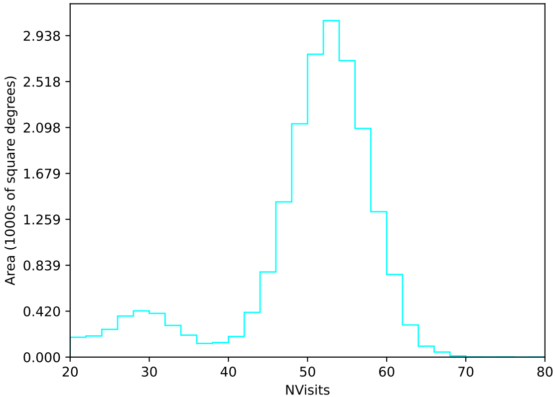
reweight_plane_v3.3_10yrs All sky u band: NVisits
