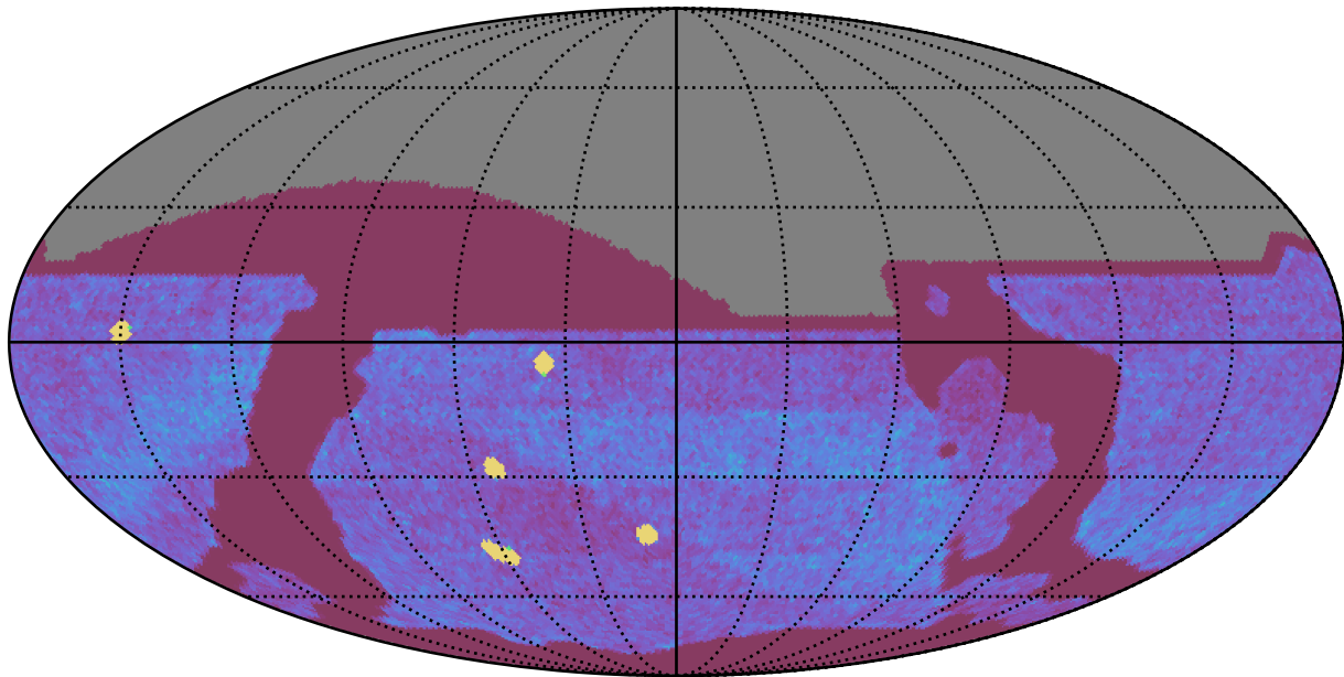
reweight_plane_v3.3_10yrs All sky all bands: NVisits
