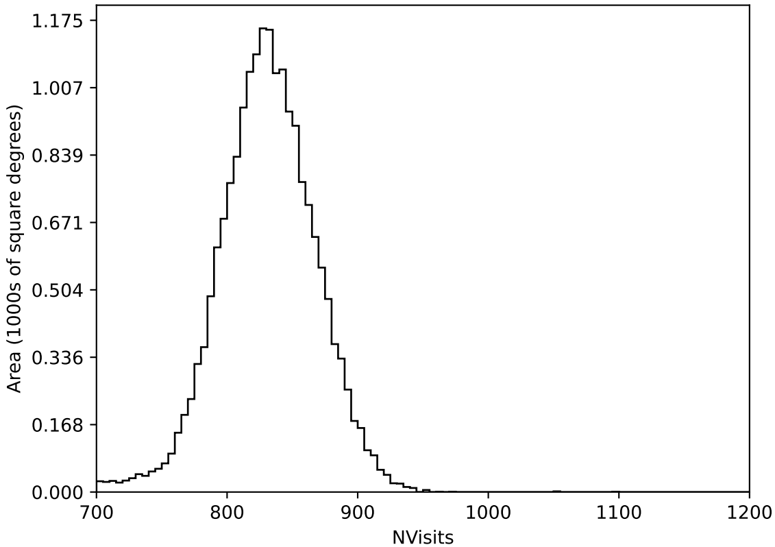
reweight_plane_v3.3_10yrs All sky all bands: NVisits
