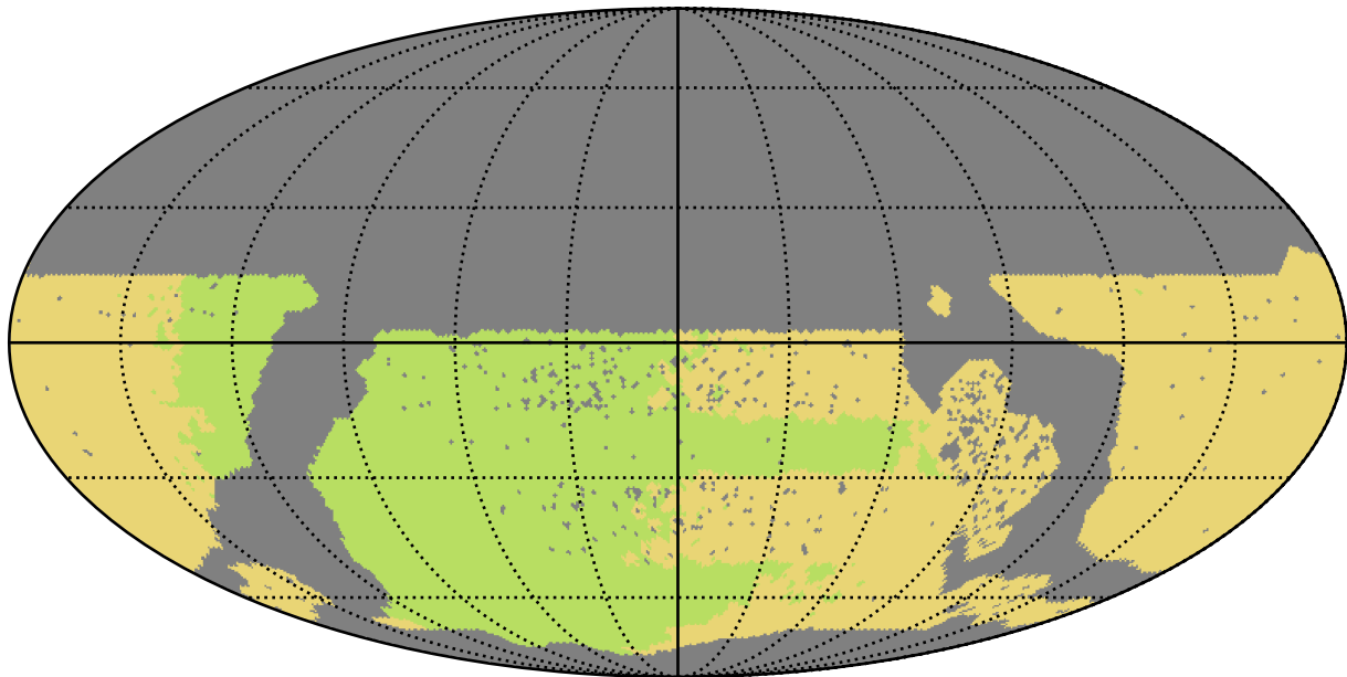
reweight_plane_v3.3_10yrs WFD all bands: NSeasons
