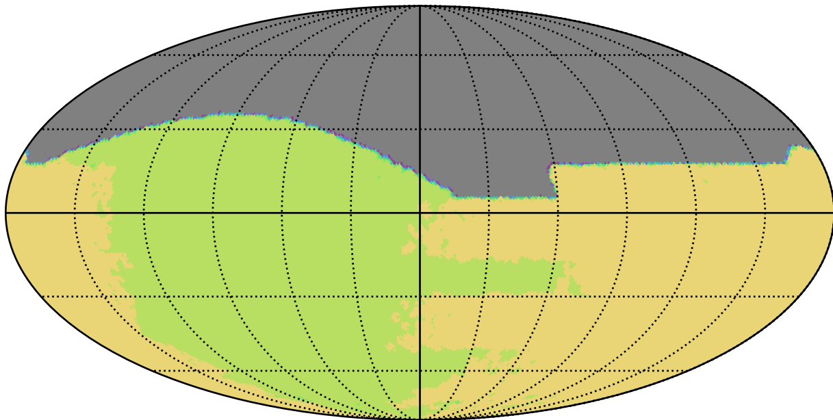
reweight_plane_v3.3_10yrs All sky all bands: NSeasons
