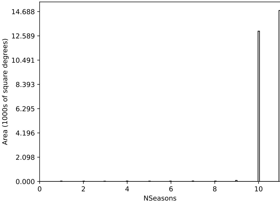
reweight_plane_v3.3_10yrs All sky all bands: NSeasons
