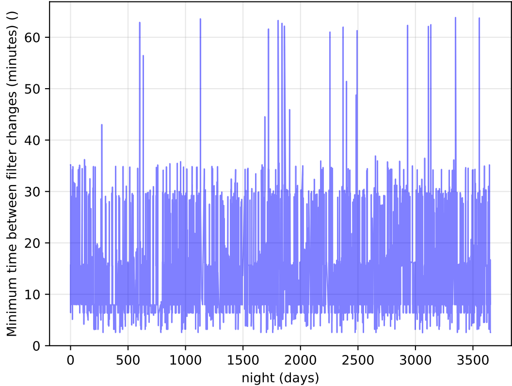
reweight_plane_v3.3_10yrs Per Night: Minimum time between filter changes (minutes)
