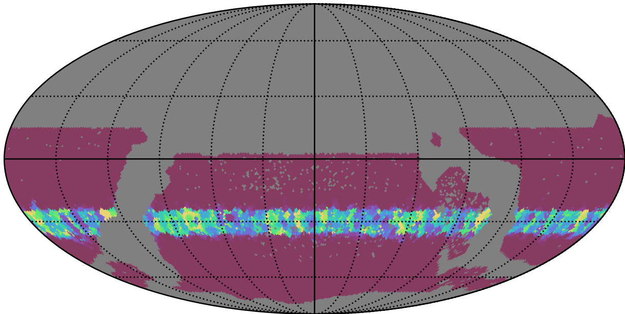
reweight_plane_v3.3_10yrs WFD z band: Min normairmass
