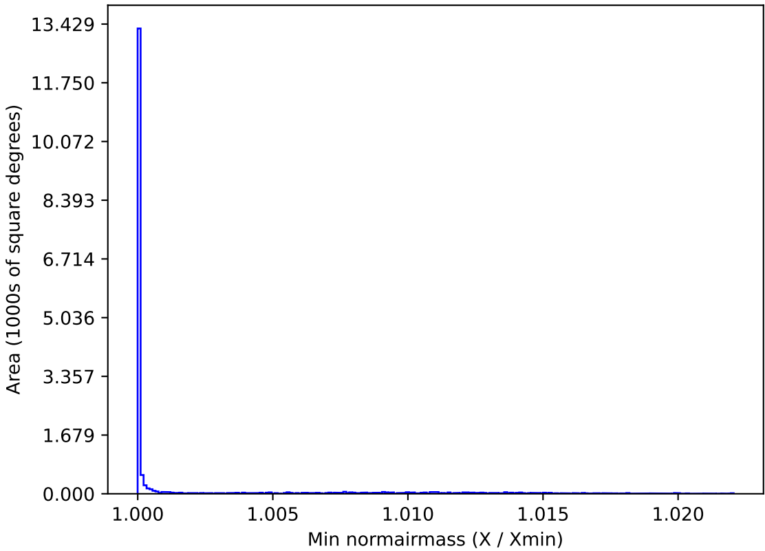
reweight_plane_v3.3_10yrs WFD z band: Min normairmass
