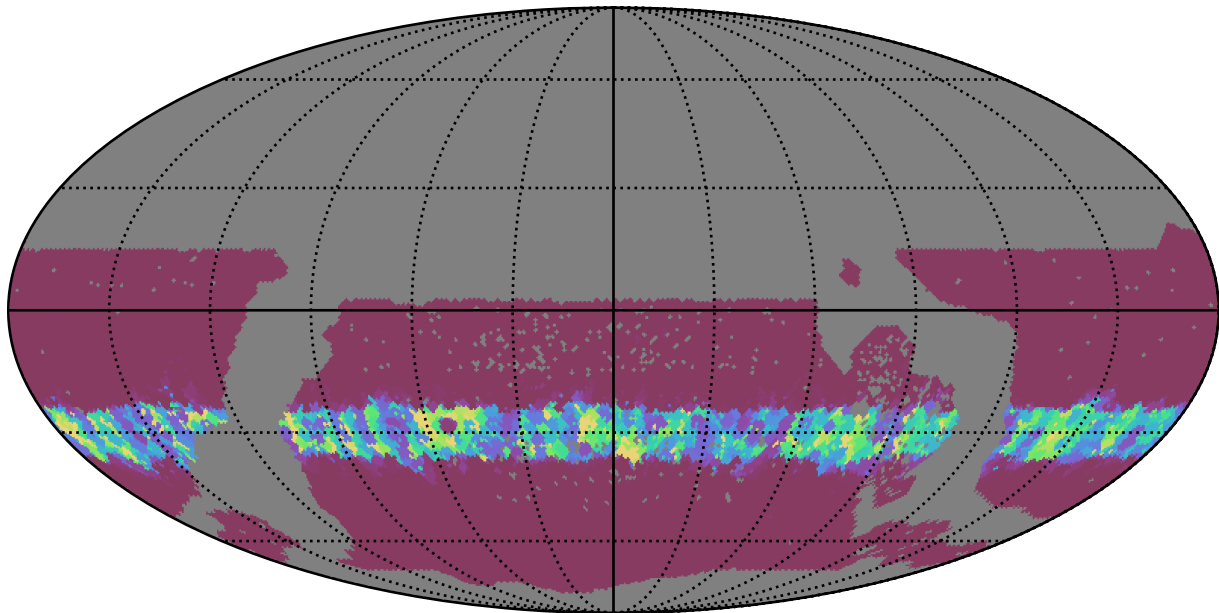
reweight_plane_v3.3_10yrs WFD y band: Min normairmass
