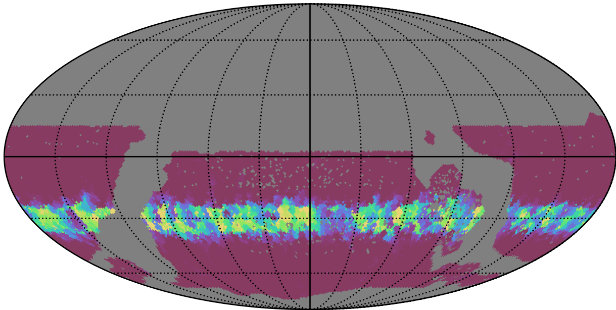
reweight_plane_v3.3_10yrs WFD u band: Min normairmass
