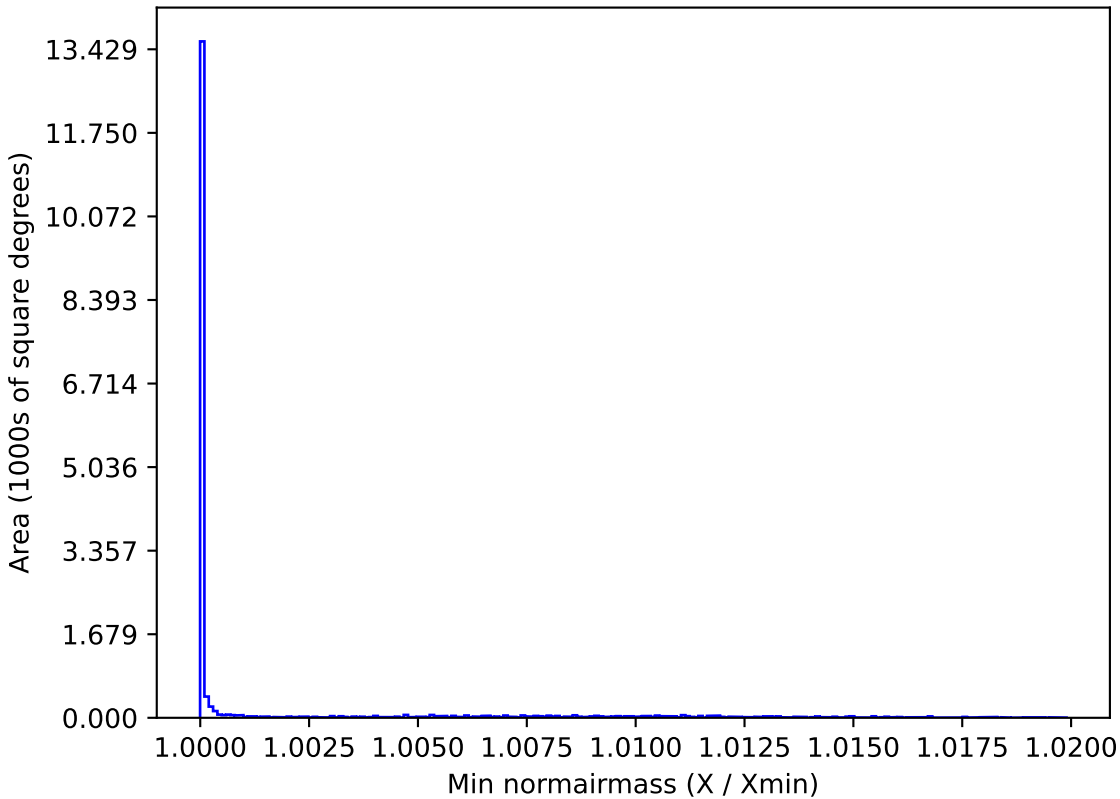
reweight_plane_v3.3_10yrs WFD r band: Min normairmass
