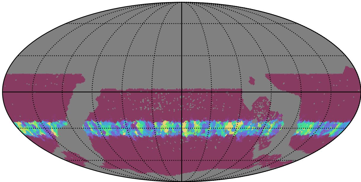
reweight_plane_v3.3_10yrs WFD i band: Min normairmass
