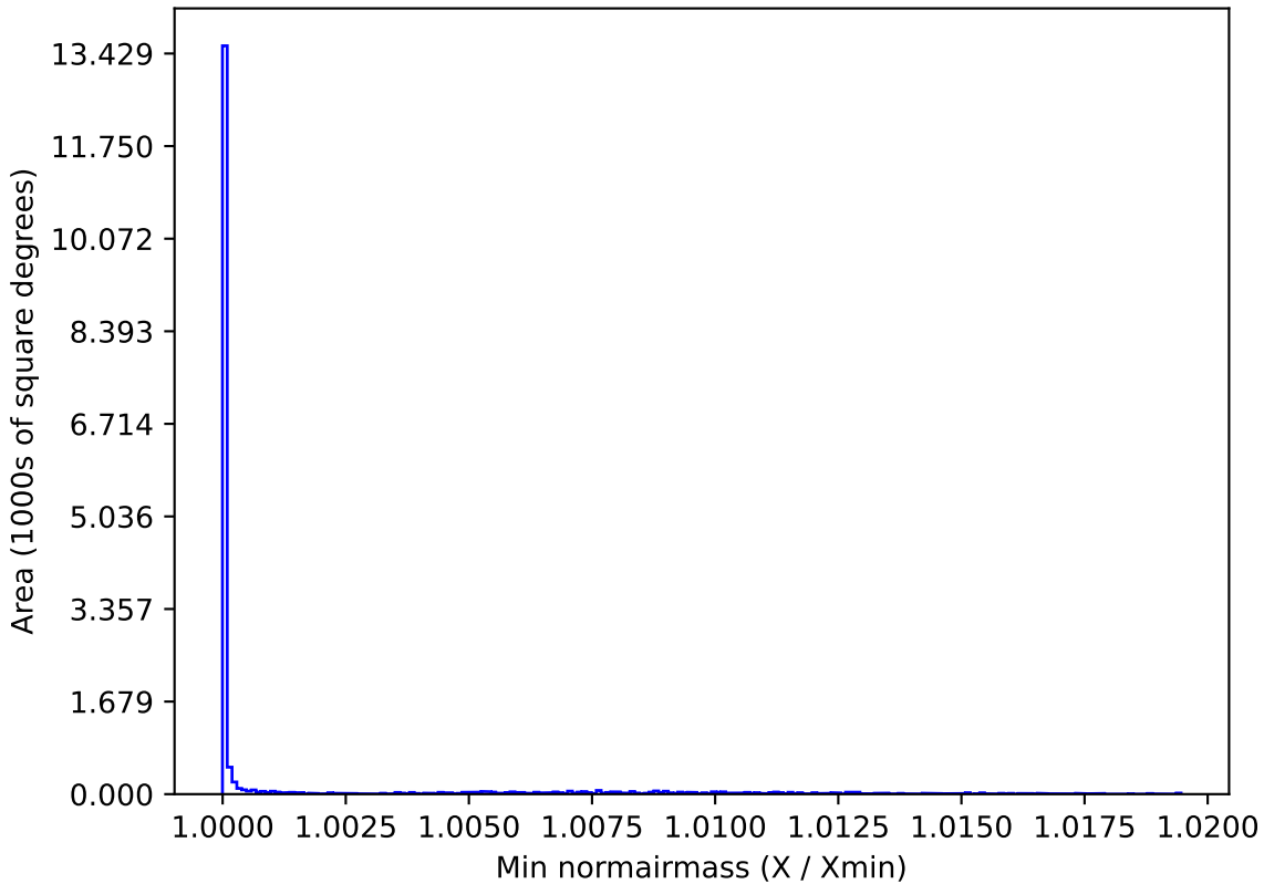
reweight_plane_v3.3_10yrs WFD i band: Min normairmass
