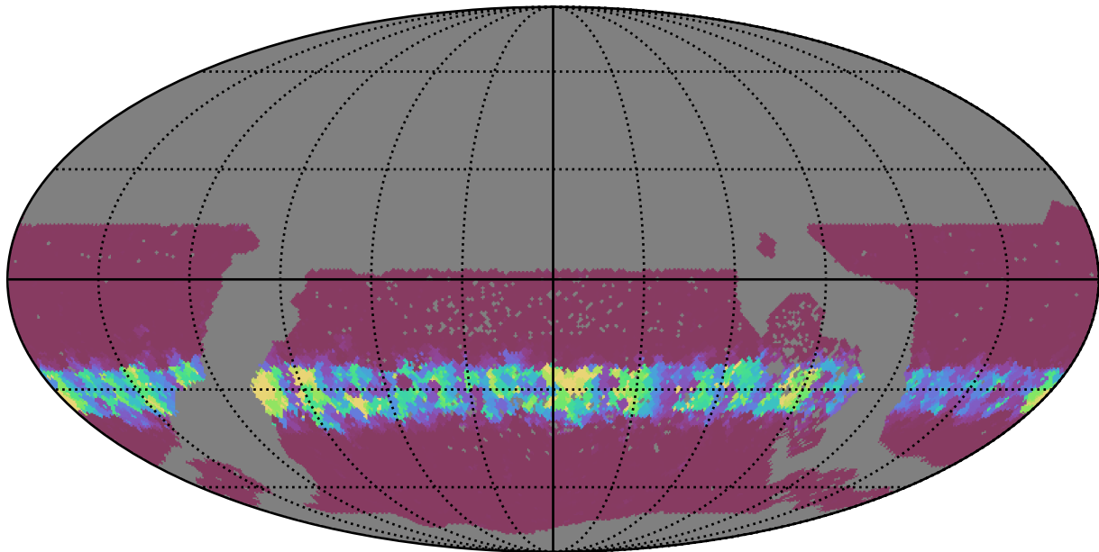
reweight_plane_v3.3_10yrs WFD g band: Min normairmass
