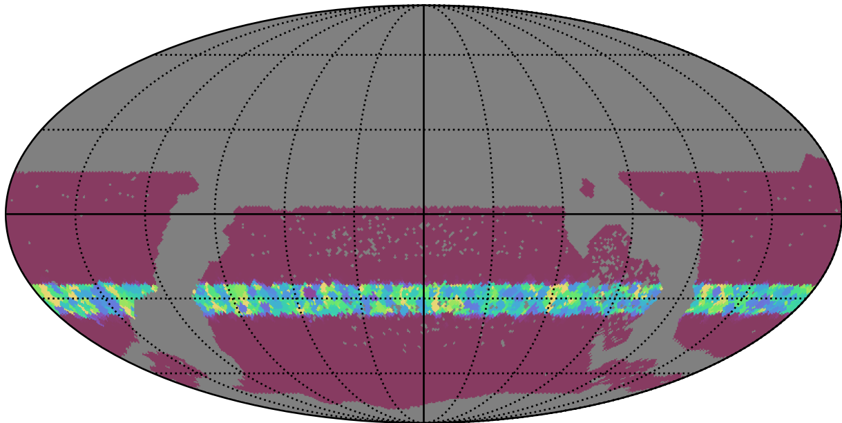
reweight_plane_v3.3_10yrs WFD all bands: Min normairmass
