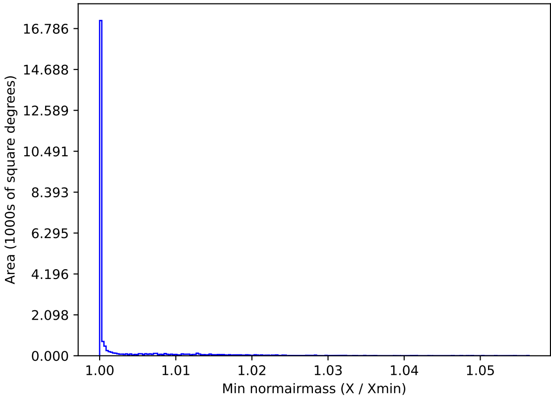
reweight_plane_v3.3_10yrs All sky y band: Min normairmass
