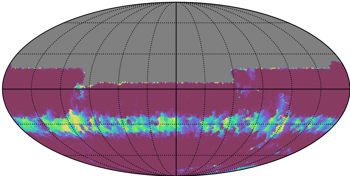
reweight_plane_v3.3_10yrs All sky u band: Min normairmass
