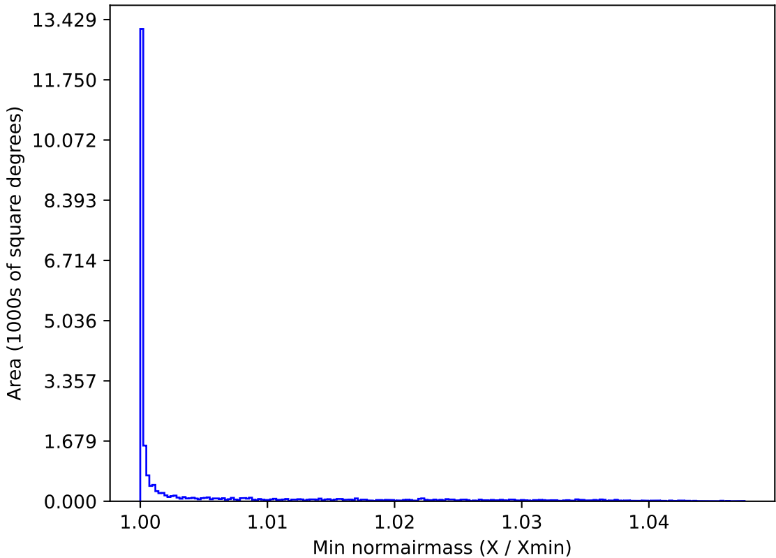
reweight_plane_v3.3_10yrs All sky u band: Min normairmass
