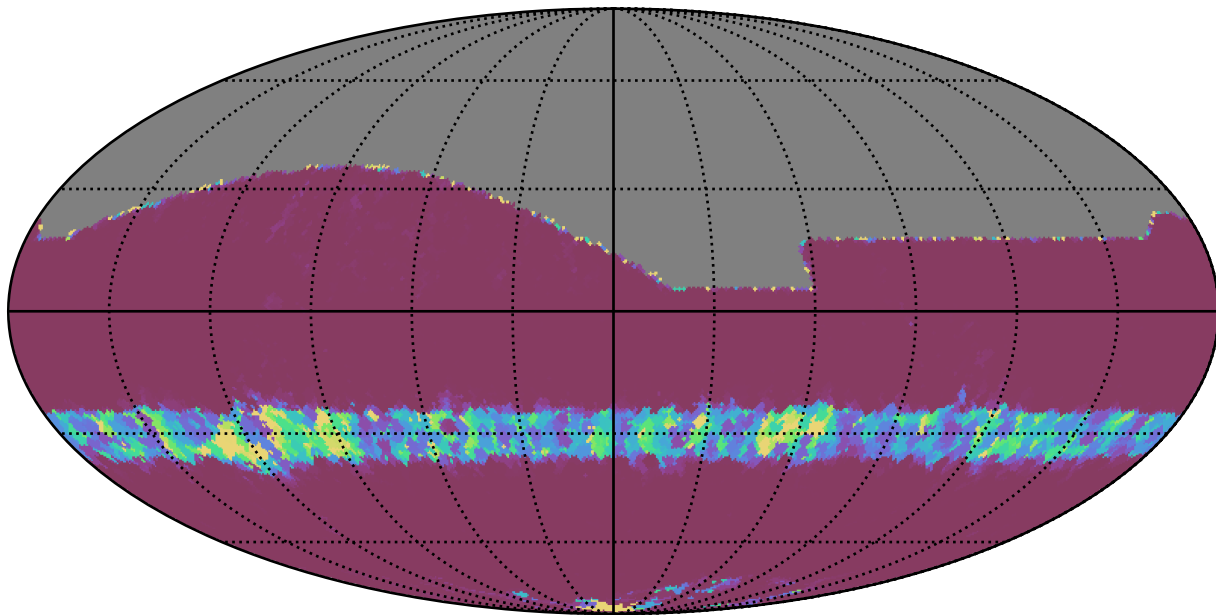
reweight_plane_v3.3_10yrs All sky r band: Min normairmass
