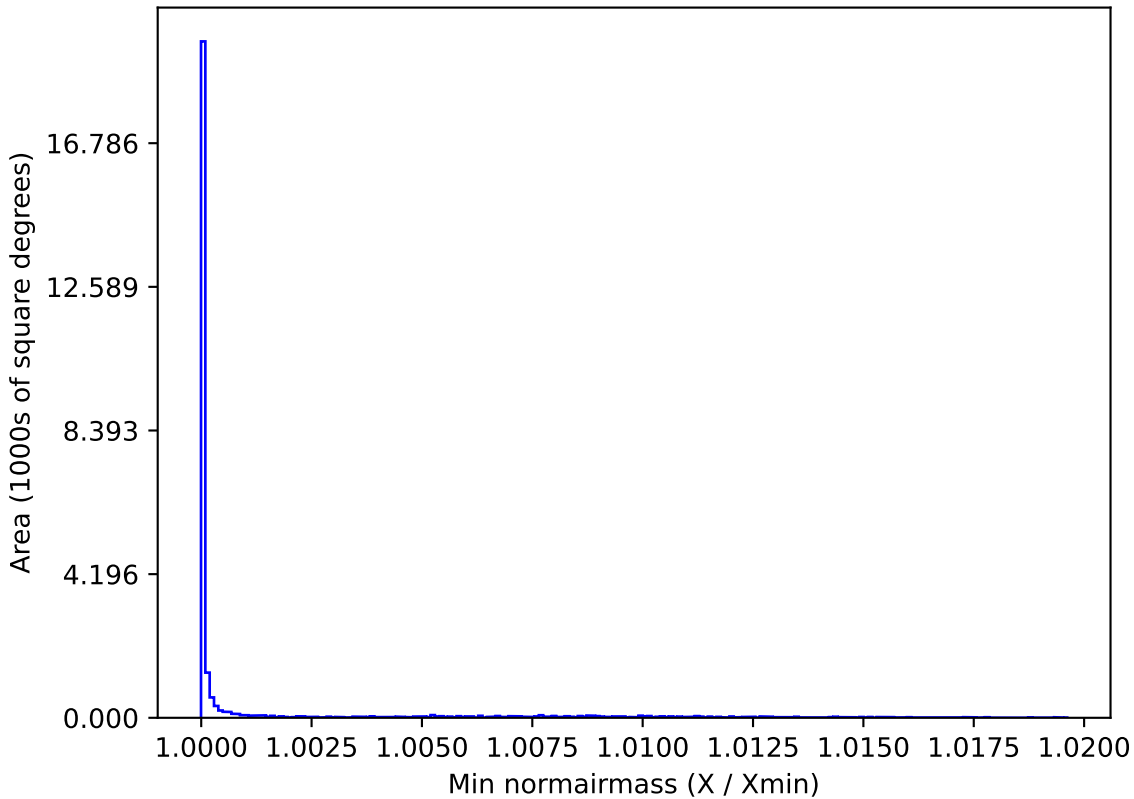
reweight_plane_v3.3_10yrs All sky i band: Min normairmass
