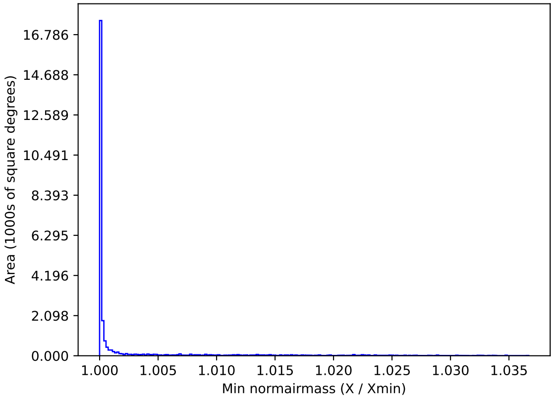
reweight_plane_v3.3_10yrs All sky g band: Min normairmass
