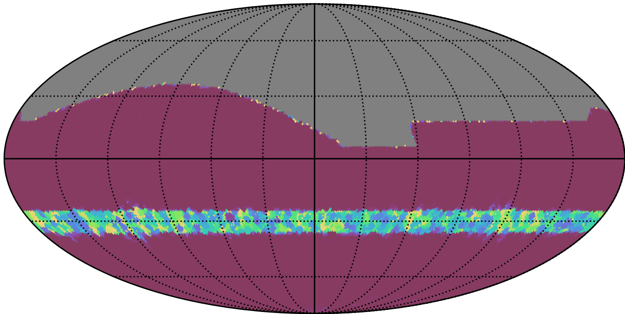
reweight_plane_v3.3_10yrs All sky all bands: Min normairmass
