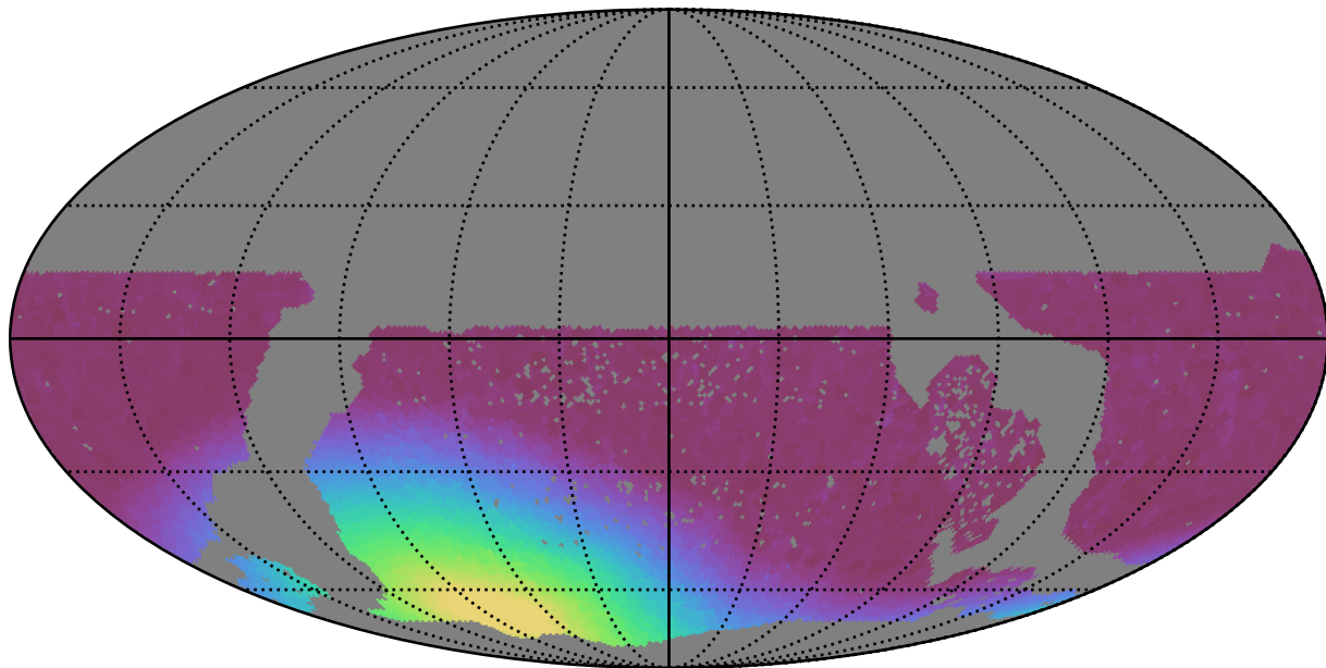
reweight_plane_v3.3_10yrs WFD z band: Min moonDistance
