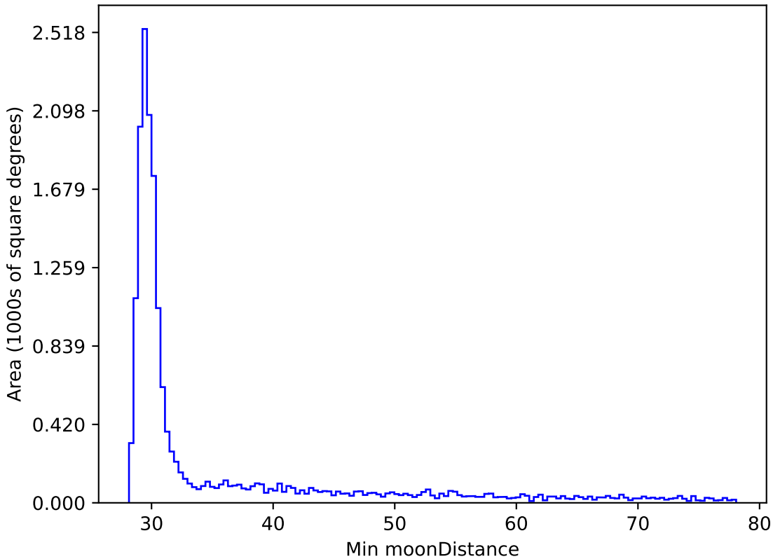
reweight_plane_v3.3_10yrs WFD z band: Min moonDistance
