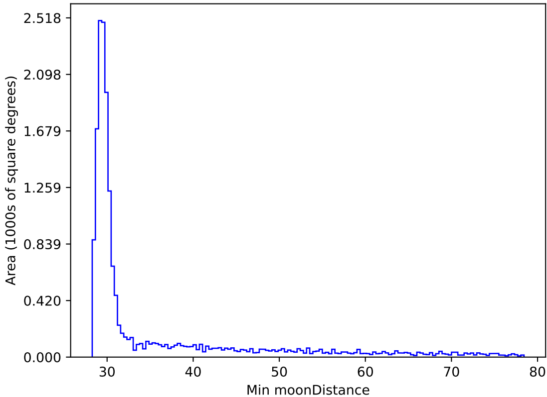
reweight_plane_v3.3_10yrs WFD y band: Min moonDistance
