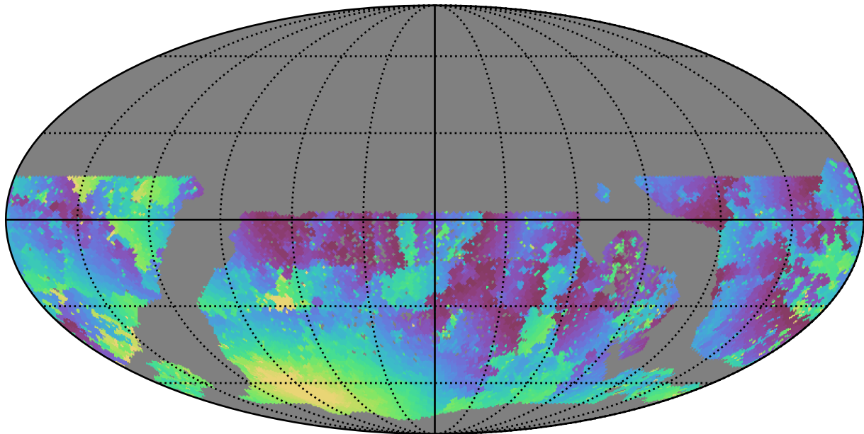
reweight_plane_v3.3_10yrs WFD u band: Min moonDistance
