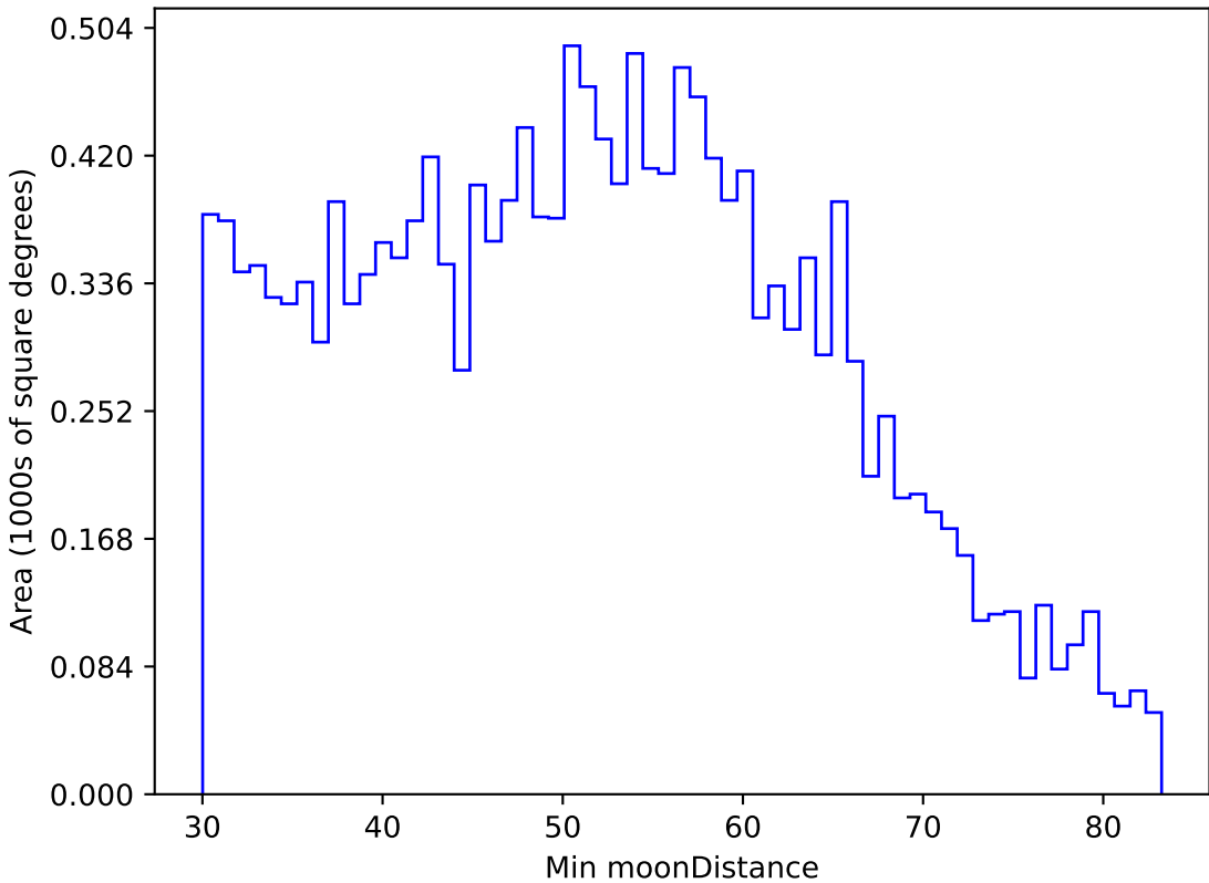
reweight_plane_v3.3_10yrs WFD u band: Min moonDistance
