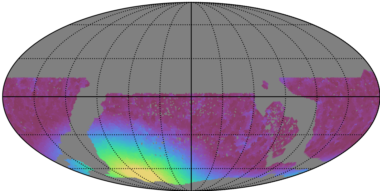
reweight_plane_v3.3_10yrs WFD r band: Min moonDistance
