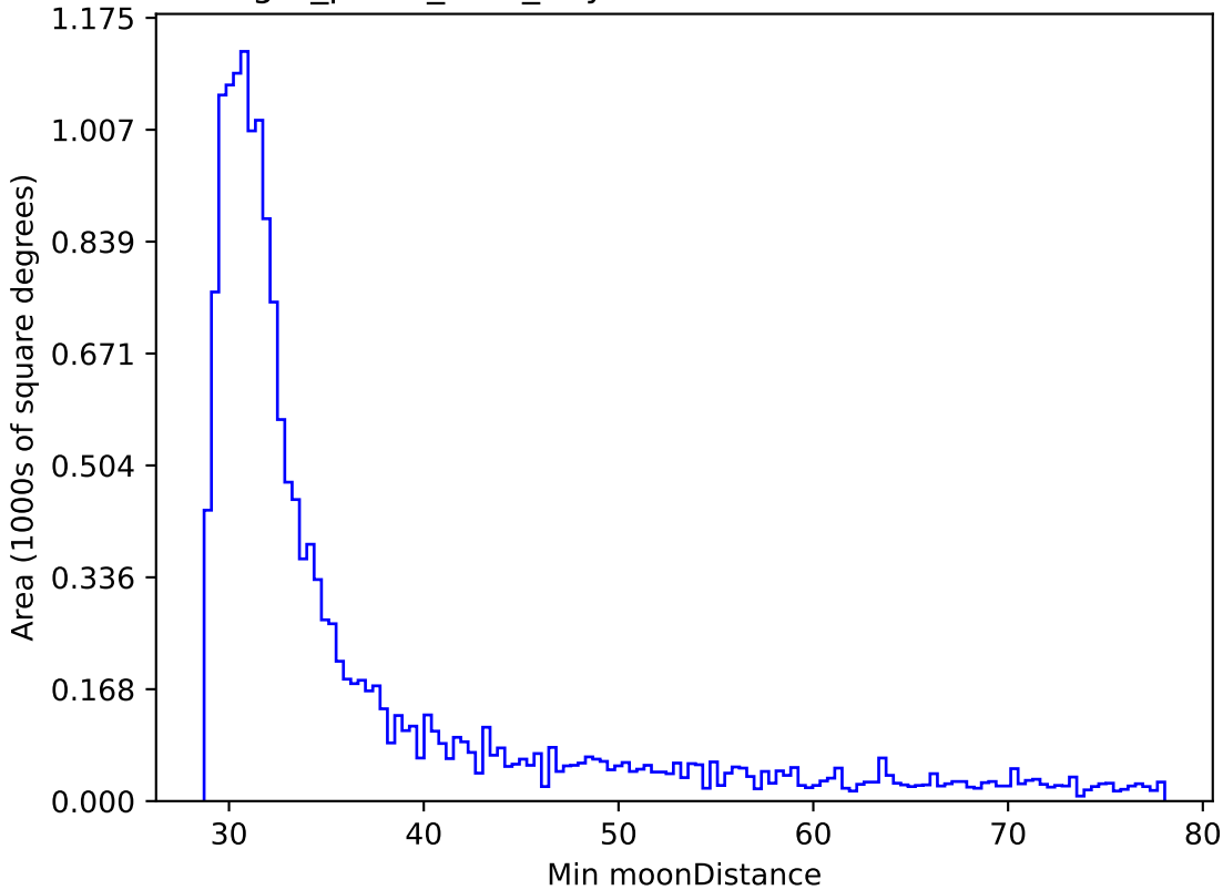
reweight_plane_v3.3_10yrs WFD r band: Min moonDistance
