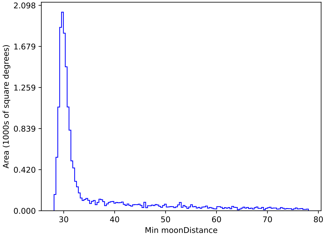
reweight_plane_v3.3_10yrs WFD i band: Min moonDistance
