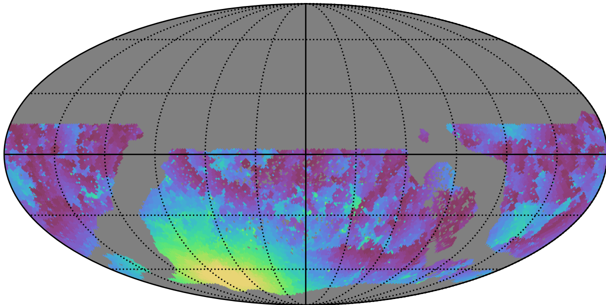
reweight_plane_v3.3_10yrs WFD g band: Min moonDistance
