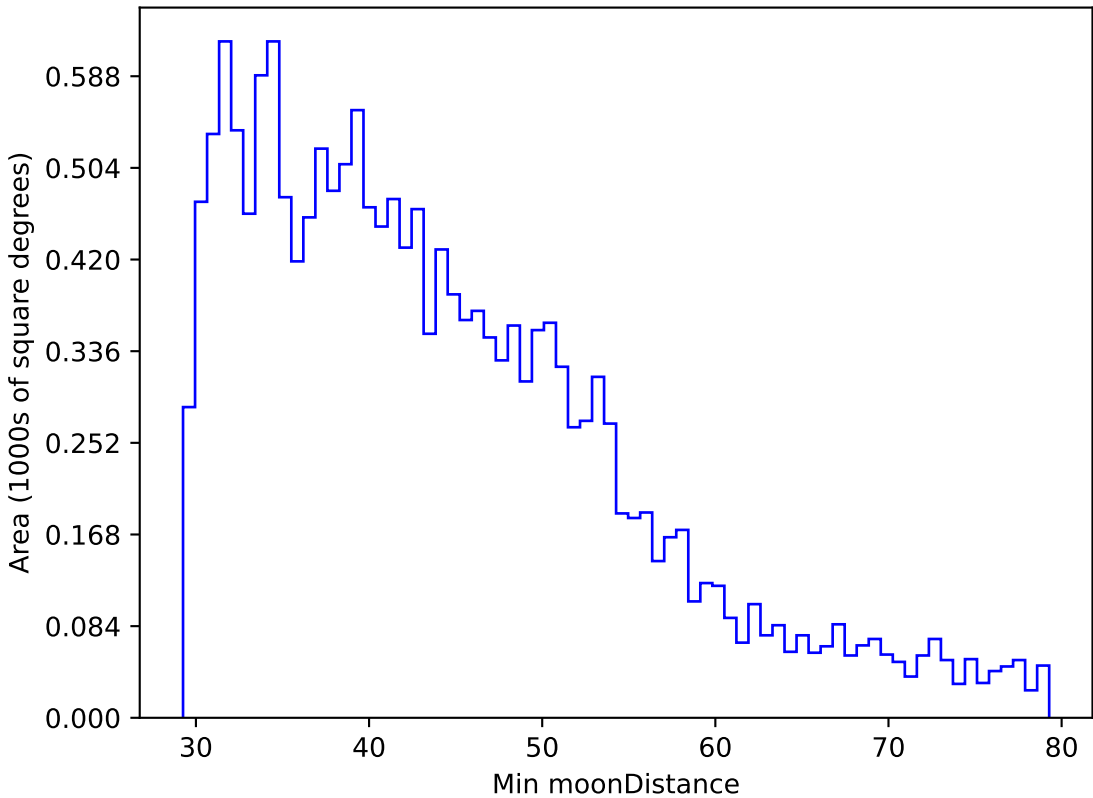
reweight_plane_v3.3_10yrs WFD g band: Min moonDistance
