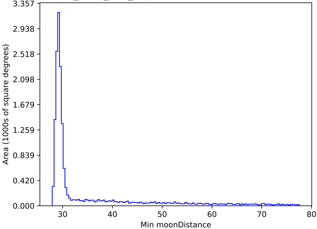
reweight_plane_v3.3_10yrs WFD all bands: Min moonDistance
